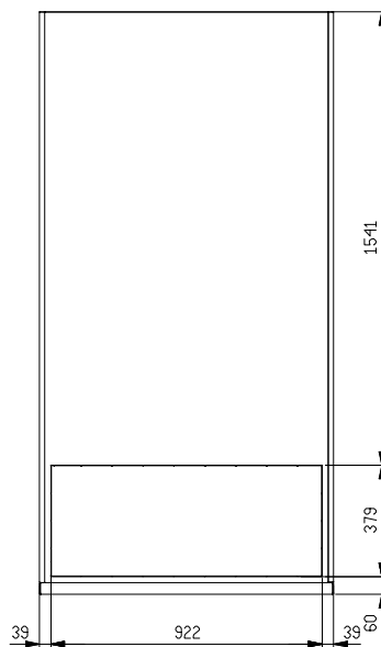
OPTION REAR AIR INTAKE
